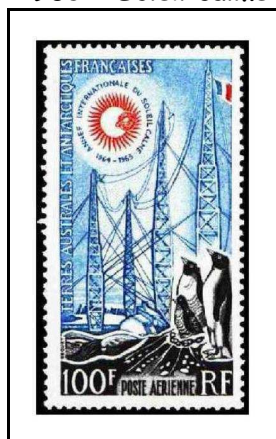
1963 - Soleil calme
